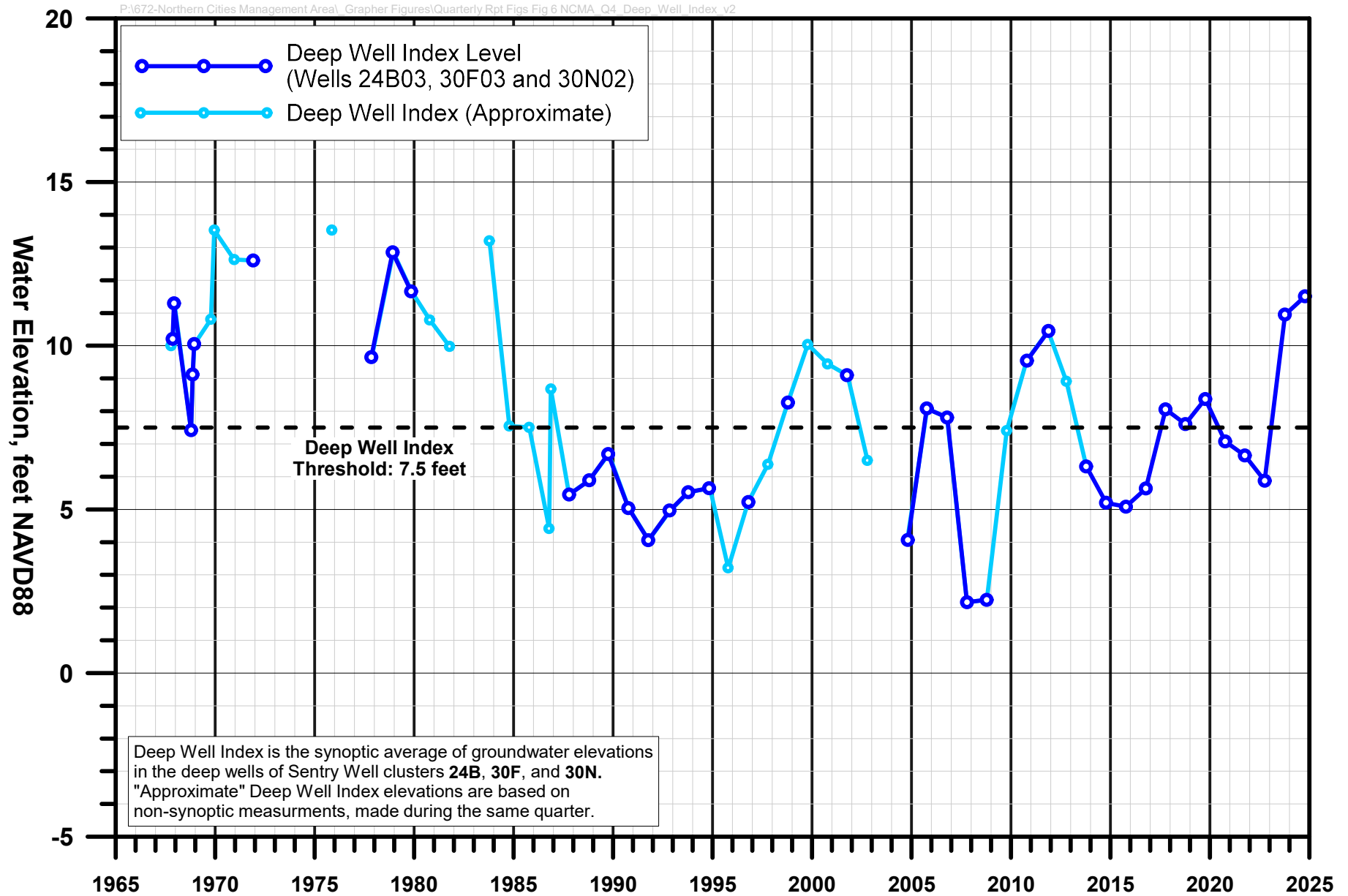
HISTORICAL FOURTH QUARTER DEEP WELL INDEX LEVELS Northern Cities Management Area San Luis Obispo County, California
