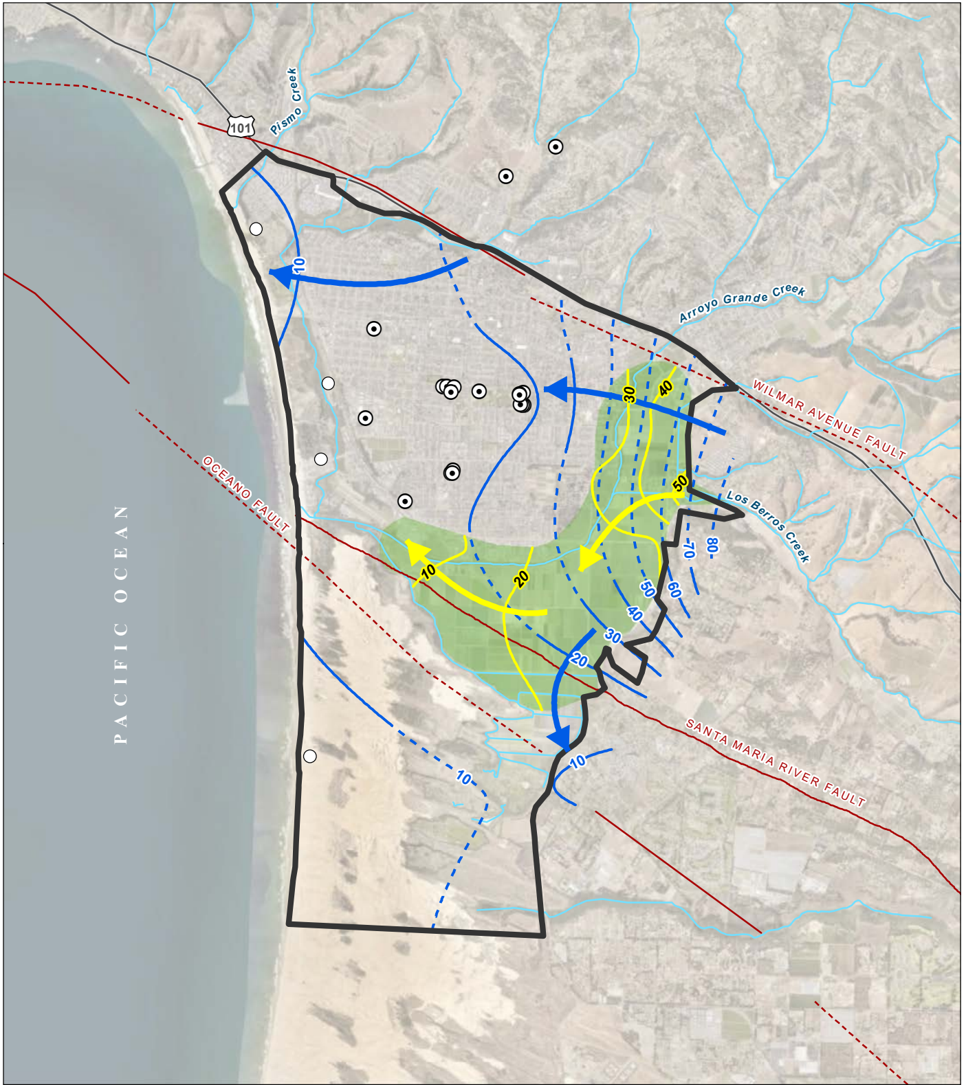
FIGURE 8 Groundwater Elevation Contours Spring 2023 Northern Cities Management Area San Luis Obispo County, California
